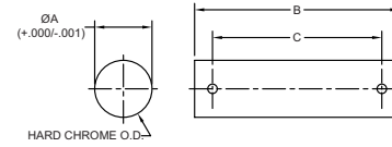
Clevis Pin
