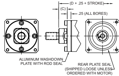
Sealed Construction (W)
